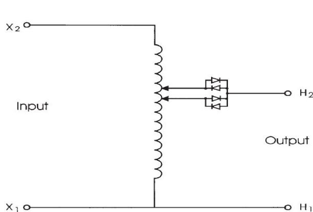
Fig.1: Single Phase, One-Coil System
