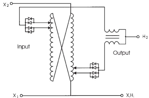
Fig.2: Single Phase, Two-Coil System
